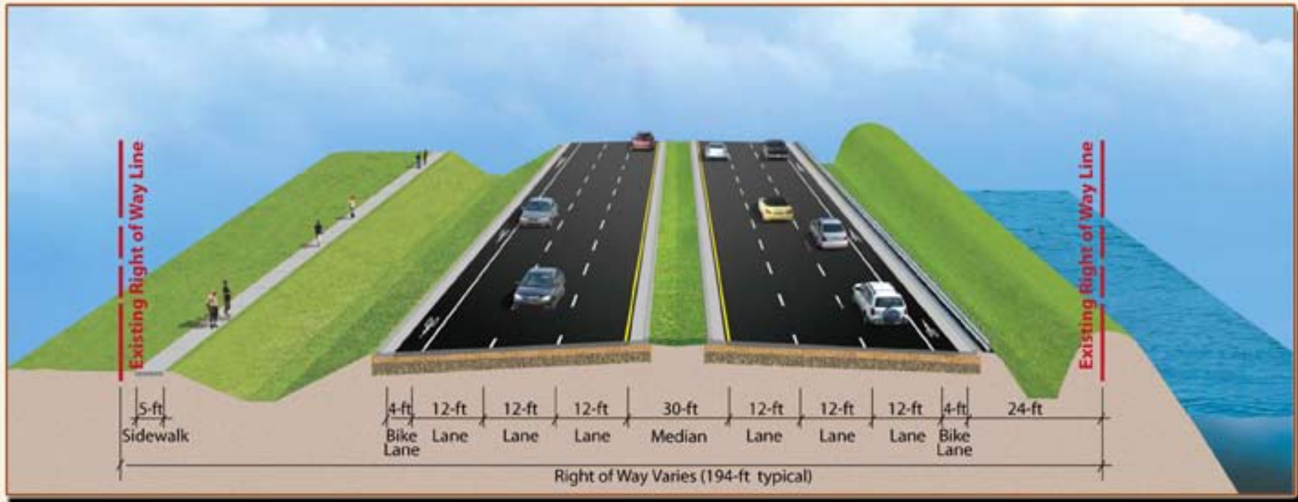
Existing 6 Lane Urban Typical Section from Palms West Parkway to Forest Hill Boulevard
