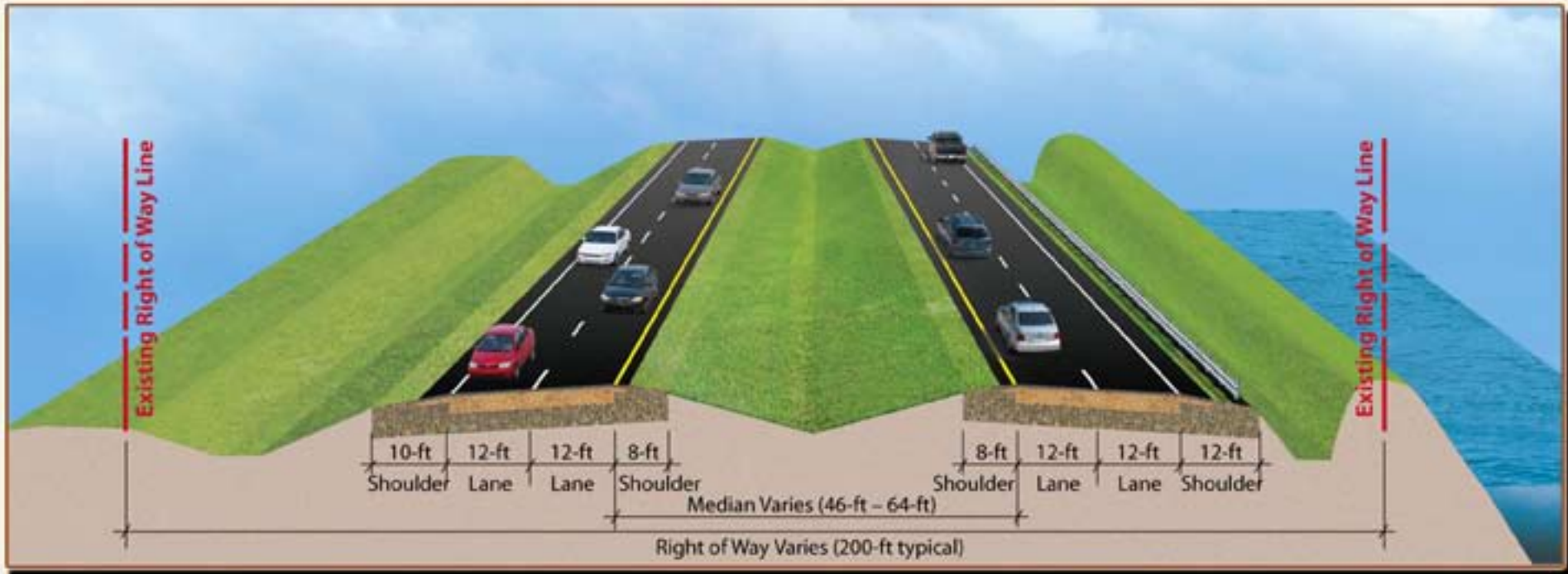
Existing 4 Lane Rural Typical Section from CR 880 to Palms West Parkway
